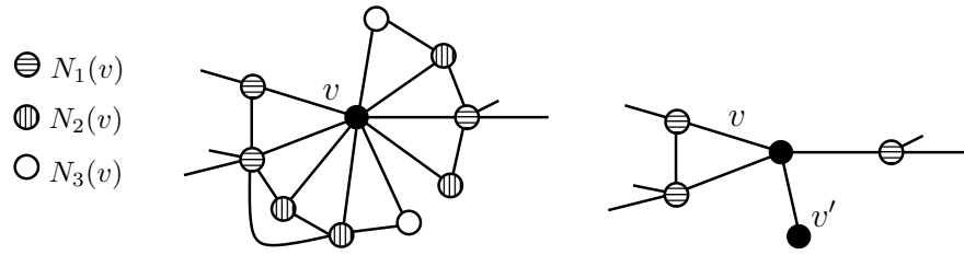
Figure 1: The left-hand side shows the partitioning of the neighborhood of a single vertex v . The right-hand side shows the result of applying Rule 1 to this particular (sub)graph.
