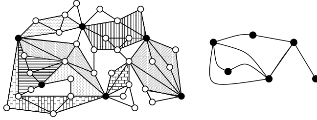
Figure 3: The left-hand side diagram shows an example of a possible D -region decomposition \mathcal{R} of some graph G , where D is the subset of vertices in G that are drawn in black. The various regions are highlighted by different patterns. The remaining white areas are not considered as regions. The given D -region decomposition is maximal. The right-hand side shows the induced graph G_{\mathcal{R}} (Definition 4).
