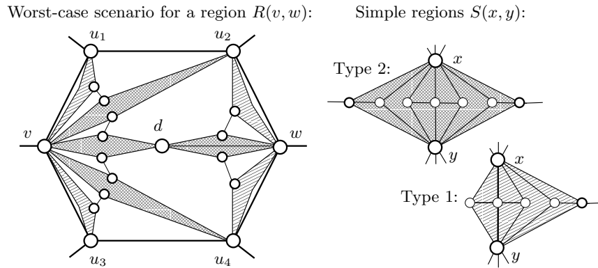
Figure 6: The left-hand diagram shows a worst-case scenario for a region R(v, w) between two vertices v and w in a reduced planar graph (cf. the proof of Proposition 3). Such a region may contain up to four vertices from N_1(v, w) , namely u_1, u_2, u_3 , and u_4 . The vertices from R(v, w) which belong to the sets N_2(v, w) and N_3(v, w) can be grouped into so-called simple regions of Type 1 (marked with a line-pattern) or of Type 2 (marked with a crossing-pattern); the structure of such simple regions S(x, y) is given in the right-hand part of the diagram. In R(v, w) there might be two simple regions S(d, v) and S(d, w) (of Type 2), containing vertices from N_3(v, w) . And, we can have up to six simple regions of vertices from N_2(v, w) : S(u_1, v), S(v, u_3), S(u_4, w), S(w, u_2), S(u_2, v) , and S(u_4, v) (among these, the latter two can be of Type 2 and the others are of Type 1). See the proof of Proposition 3 for details.
