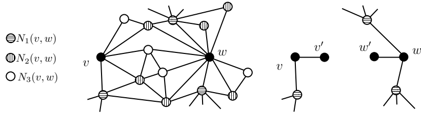
Figure 2: The left-hand side shows the partitioning of a neighborhood N(v, w) of two vertices v and w . The right-hand side shows the result of applying Rule 2, Case 2 to this particular (sub)graph.
