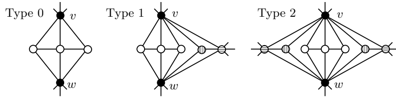
Figure 5: Simple regions of Type 0, Type 1, Type 2. This figure illustrates the largest possible simple regions in a reduced graph. Vertices marked with horizontal lines are in N_1(v, w) , vertices marked with vertical lines belong to N_2(v, w) , and white vertices are in N_3(v, w) .
